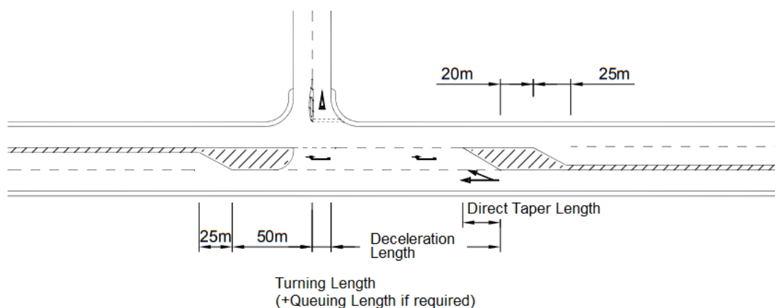
Figure 6.2c Formation of right-turn at end of overtaking lane section on WS2+1 road
